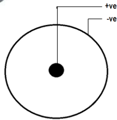
10.5 mm DC Jack Connector
